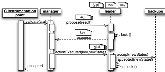
Fig. 6. Successful protocol execution
