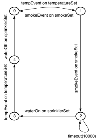
Fig. 2. The graphical form of the global FSM
