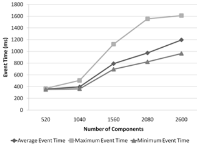
Fig. 9. Base Average Event Time Performance
